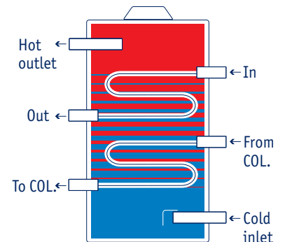
Double Spiral Heat-Exchanger (Closed-Loop system)
