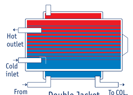
Double Jacket Heat-Exchanger (Closed-Loop system)
