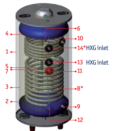
Double Spiral Solar Water Tank
