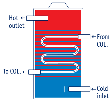
Spiral/ Serpentine Heat-Exchanger (Closed-Loop system)
