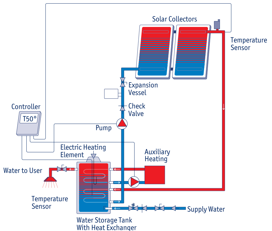
Forced circulation system - schematic
