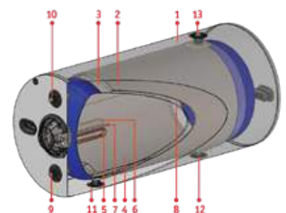
300L horizontal storage tank Double jacket heat exchanger Aluminium external envelope
