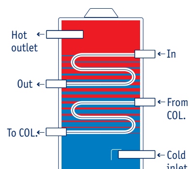
Double Spiral Heat-Exchanger (Closed-Loop system)
