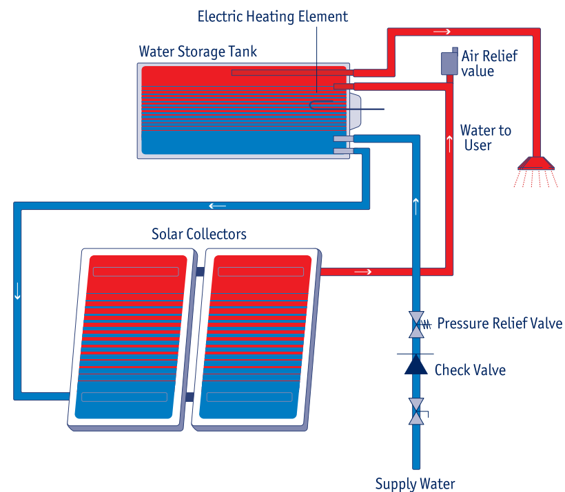
Thermosiphon open-loop system - schematic
