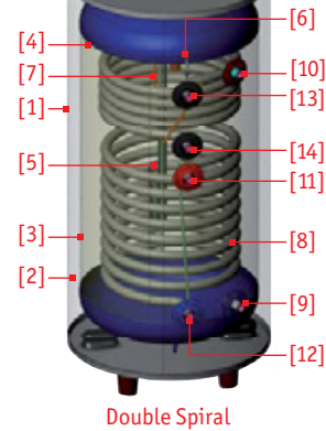
Double Spiral
