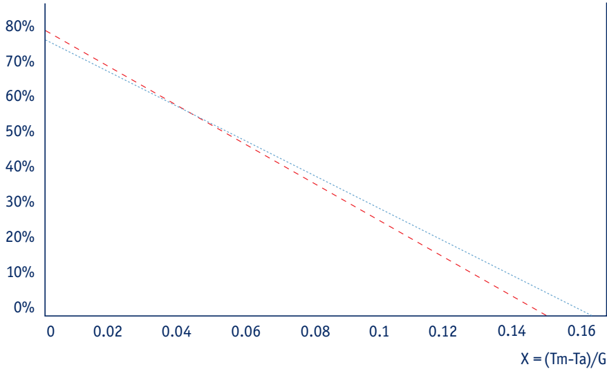
Efficiency curve
