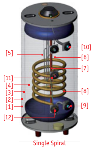
Single Spiral
