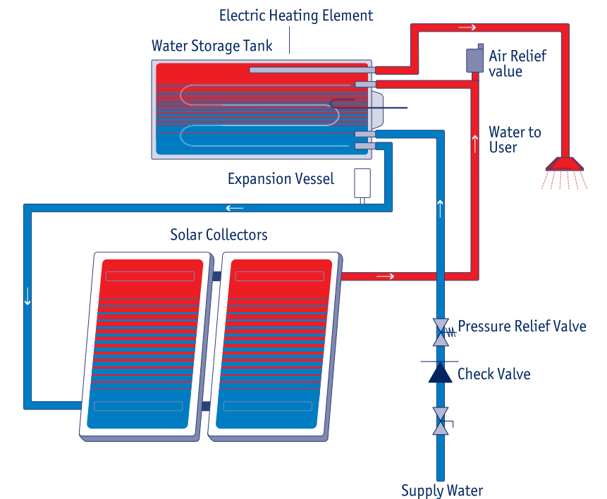
Thermosiphon closed-loop system - schematic
