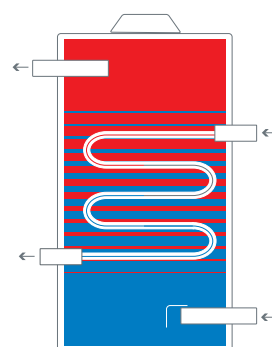
Spiral/Serpentine Heat-Exchanger (Closed-Loop System)
