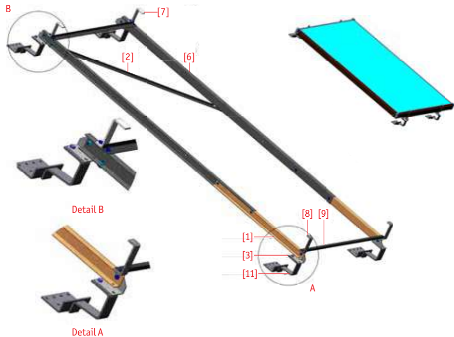
Single Collector Steel Rack
