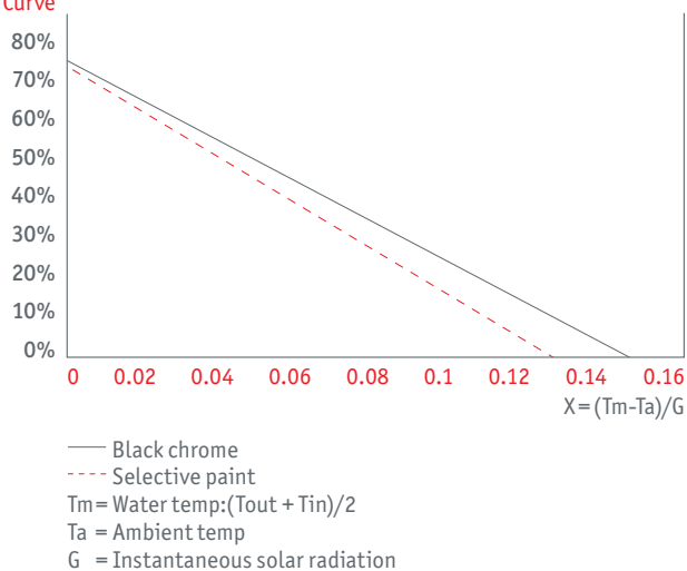
Efficiency Curve
