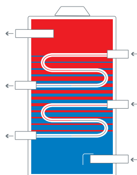
Double Spiral Heat-Exchanger (Closed-Loop System)
