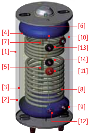
Double Spiral
