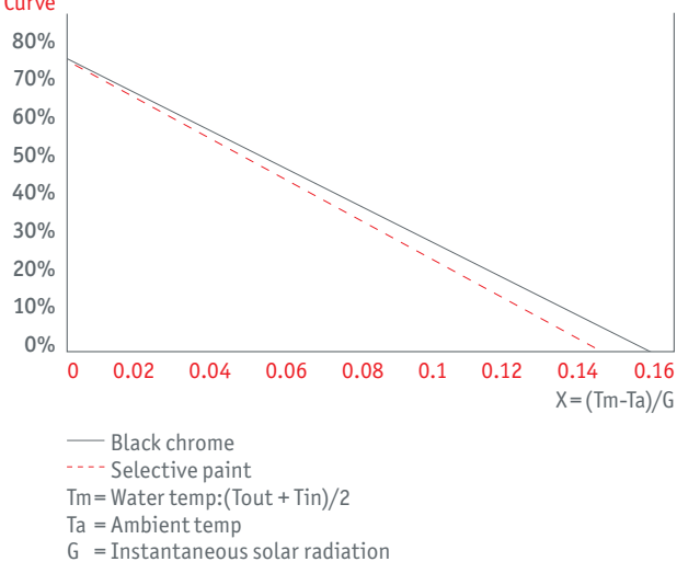
Efficiency Curve
