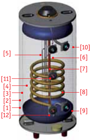
Single Spiral
