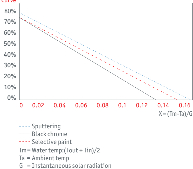
Efficiency Curve
